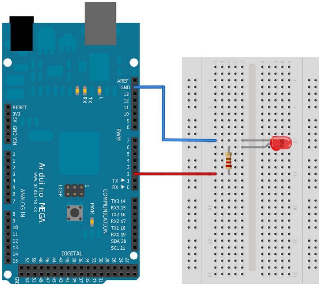
Figure 3-10. Project 1 setup
