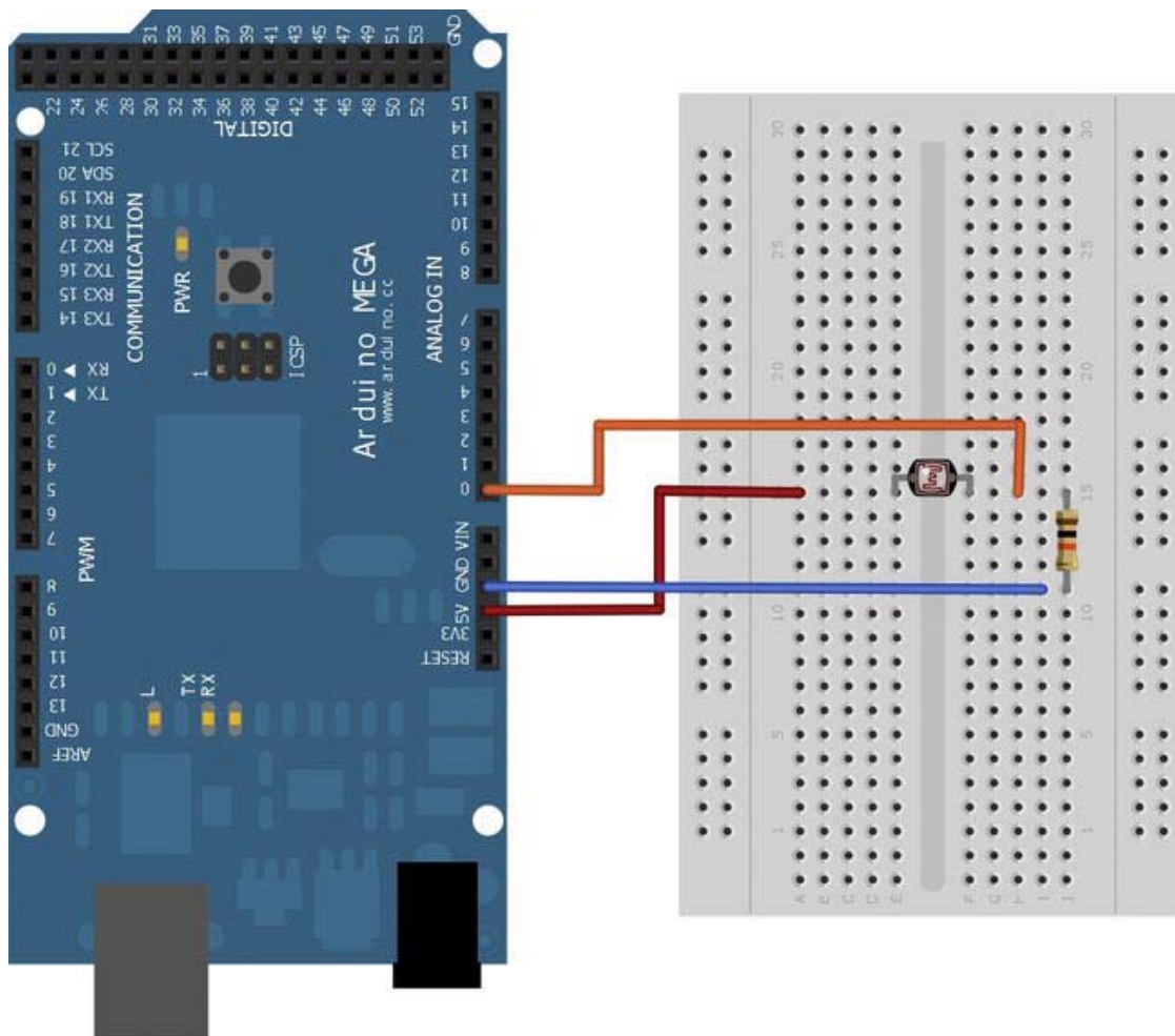
Figure 6-4. Project 7 setup
