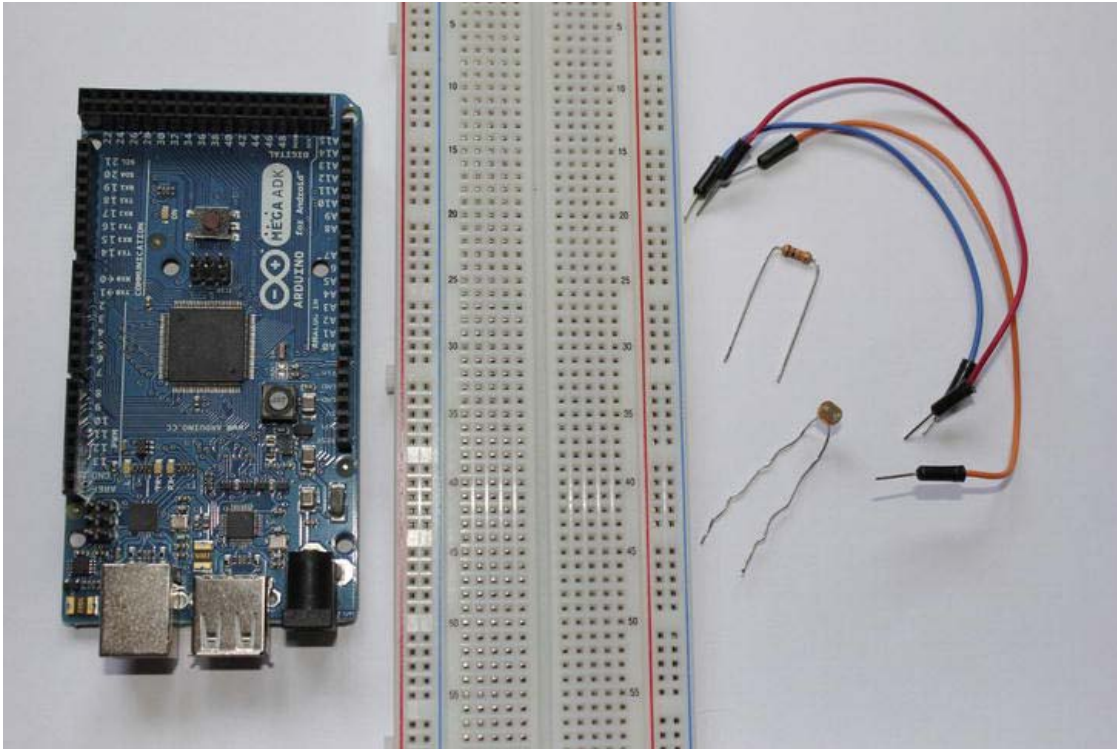
Figure 6-1. Project 7 Parts (ADK board, breadboard, wires, photoresistor, 10kΩ resistor)
