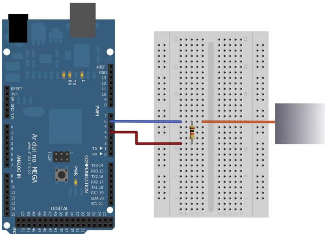
Figure 8-6. Project 9 setup
