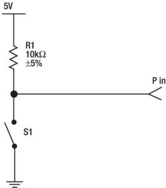
Figure 4-5. Pull-up resistor circuit
