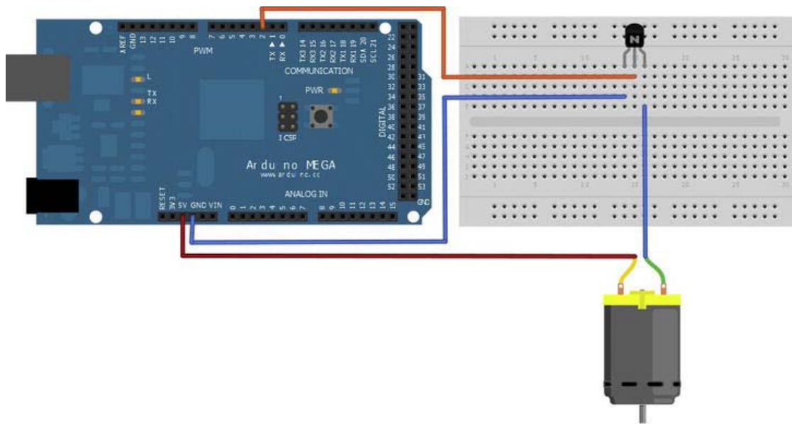
Figure 9-15. Project 11 setup
