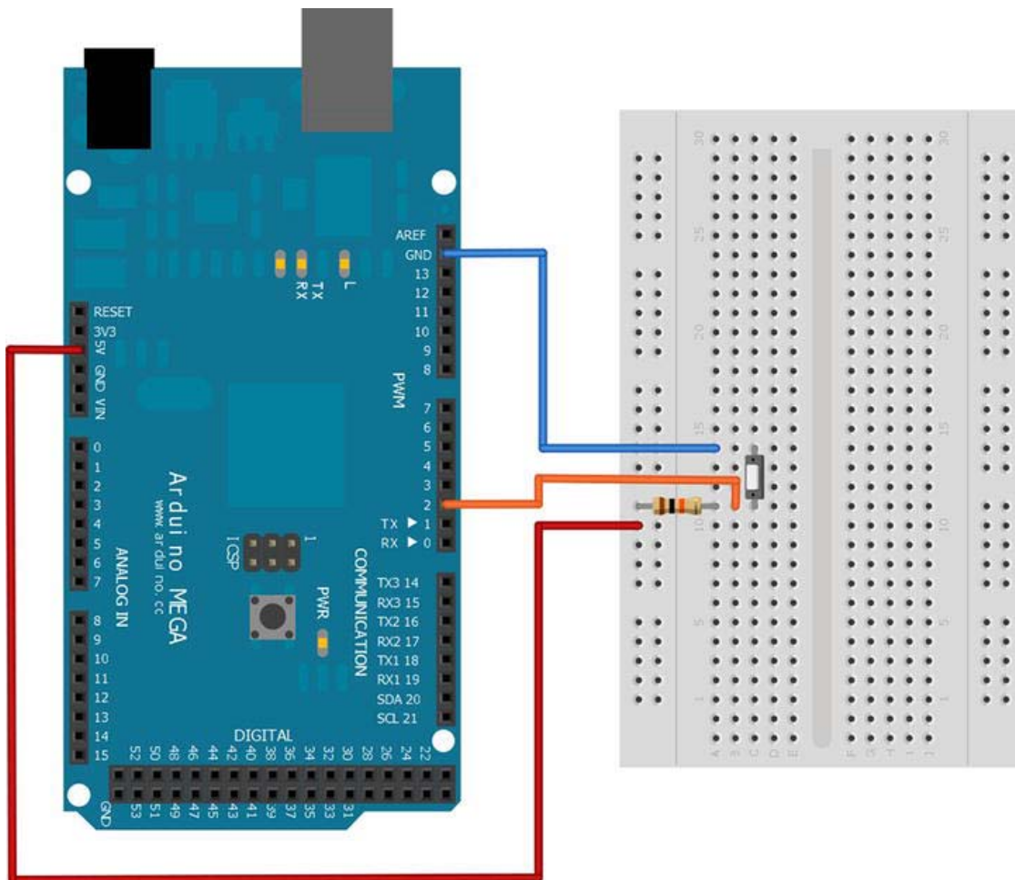
Figure 4-6. Project 3 setup
