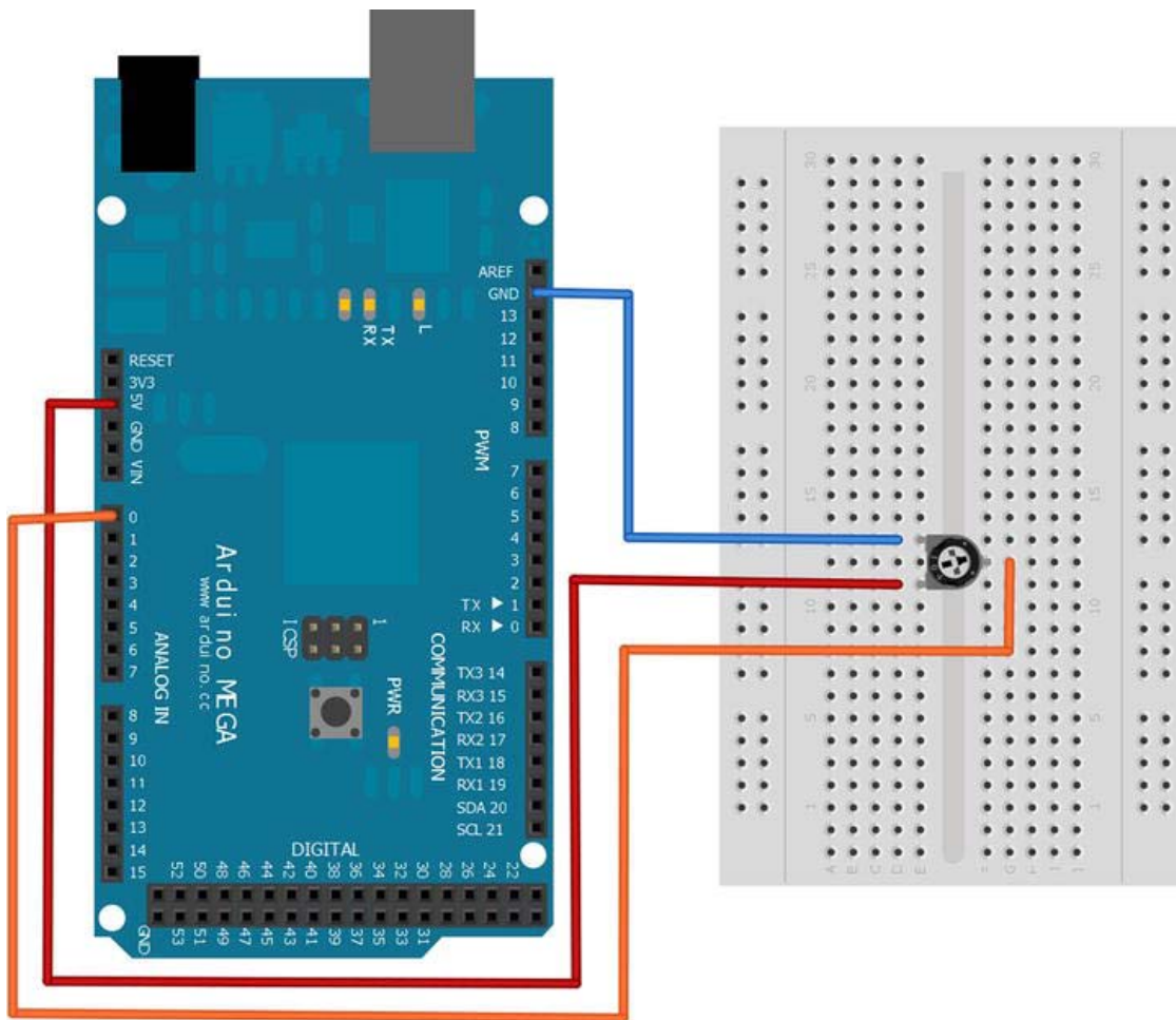
Figure 4-13. Project 4 setup
