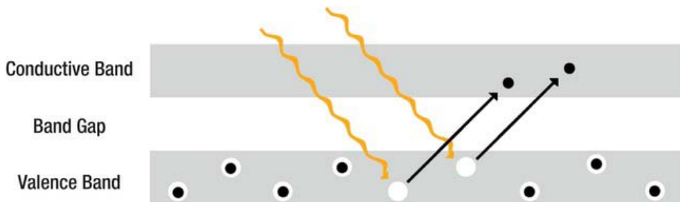
Figure 6-3. Photoelectric effect
