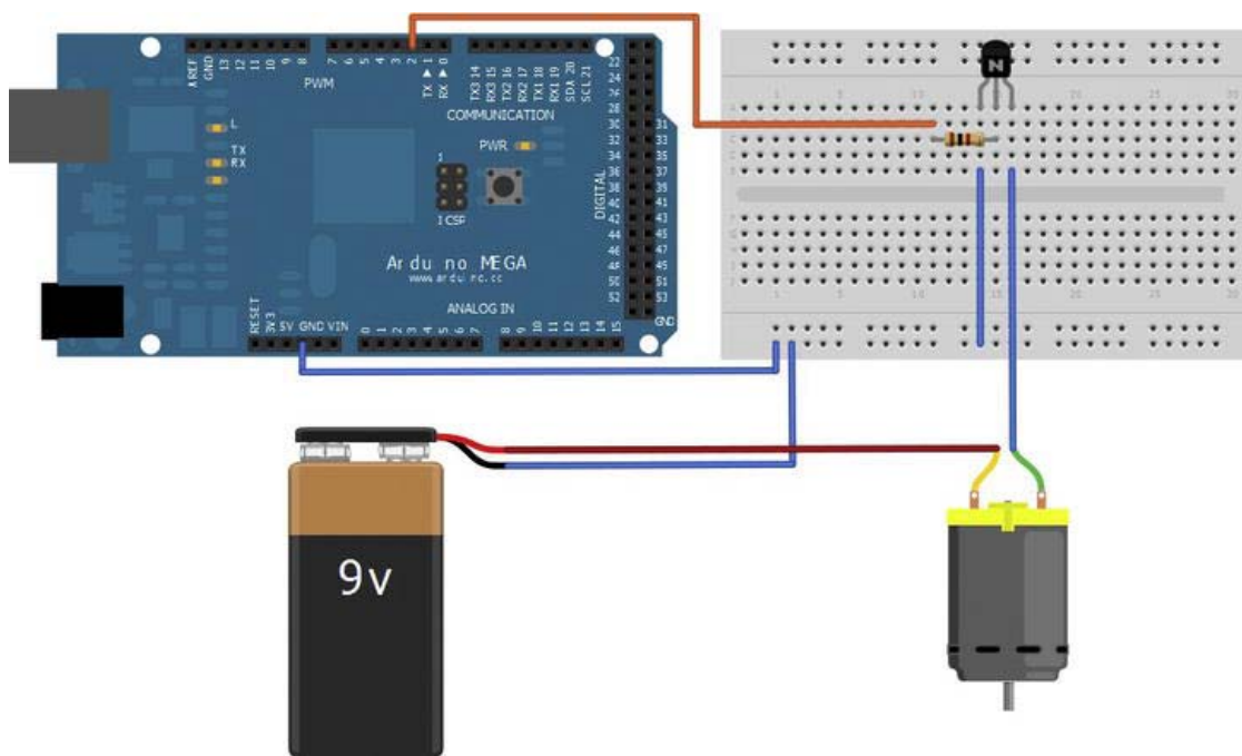
Figure 9-16. Project 11 setup with external battery
