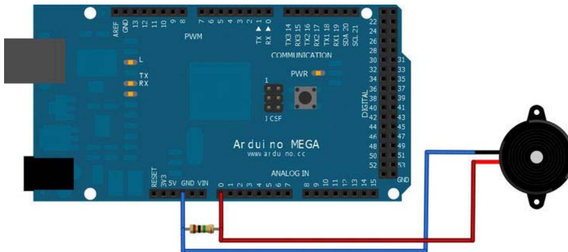
Figure 5-8. Project 6 setup
