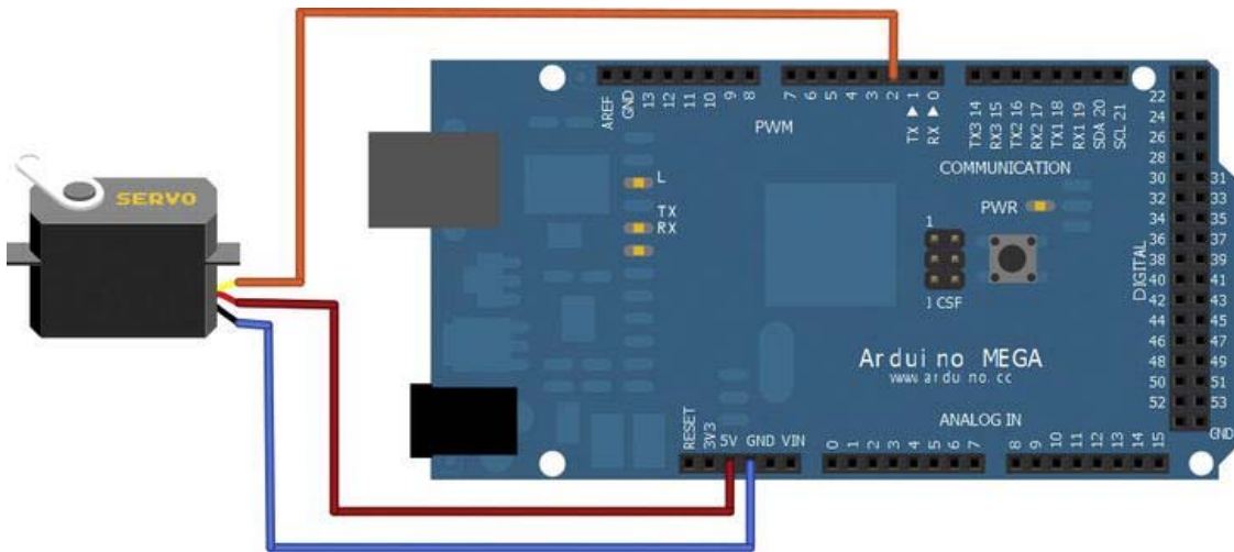
Figure 9-7. Project 10 setup
