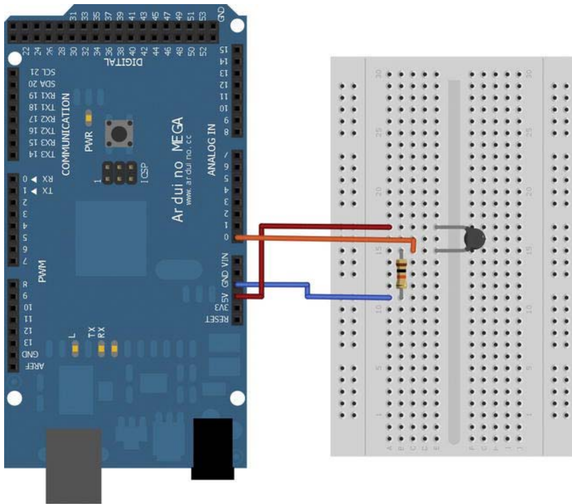
Figure 7-5. Project 8 setup
