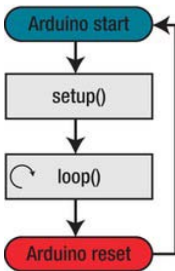
Figure 2-4. Sketch lifecycle
