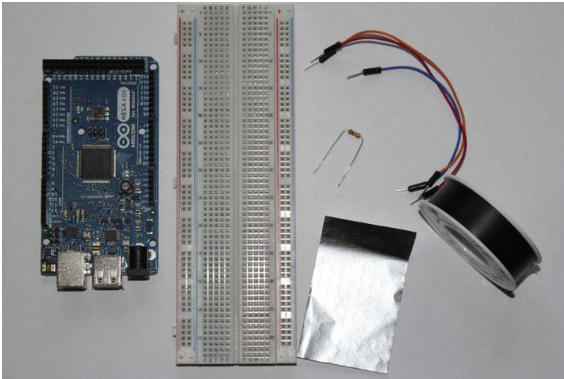
Figure 8-1. Project 9 parts (ADK board, breadboard, wires, aluminum foil, adhesive tape, 10kΩ resistor)
